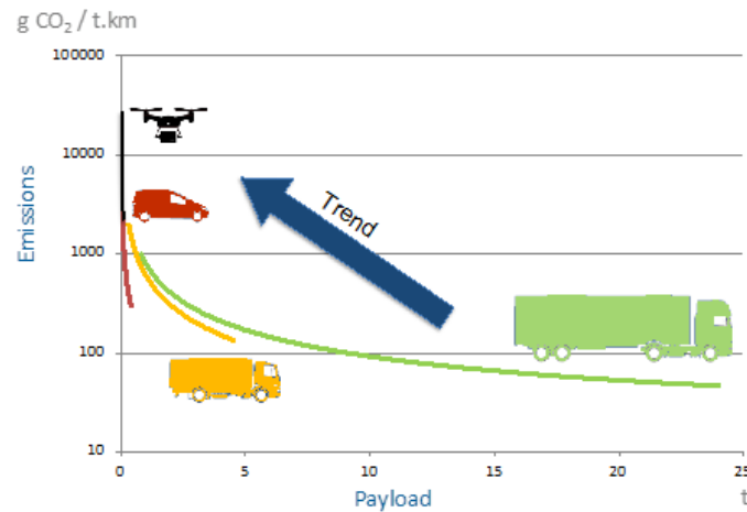
Figure 5 - CO 2 emission per tonne.km according to the payload and vehicle: data sources 57
